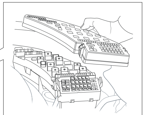
REAR POWER DISTRIBUTION FUSE BOX
