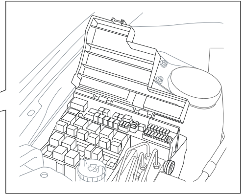
FRONT POWER DISTRIBUTION FUSE BOX
